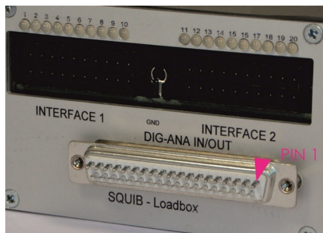
37-pole SUB-D Plug
